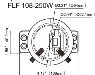
Slipfitter Mount for FLF 108-250W
