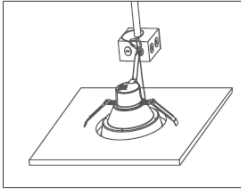
Ensure fixture is flush. Installation is complete
